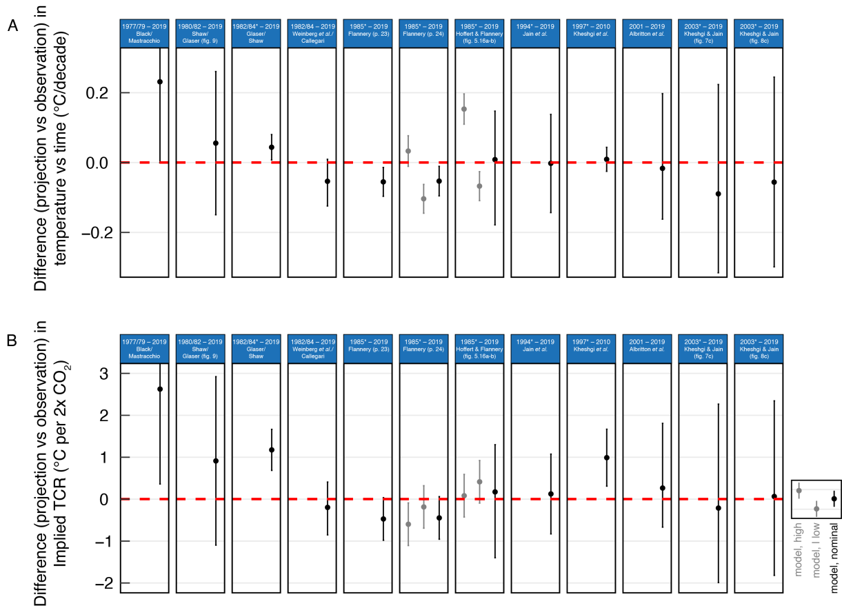
Fig. S1. Differences between (i) historical observations and (ii) projections reported by ExxonMobil scientists in internal documents and peer-reviewed publications in terms of (A) temperature change versus time and (B) temperature change versus change in radiative forcing (“implied TCR”). Differences are computed over model projection periods indicated in the blue boxes above each panel. Asterisks indicate global warming projections modeled by ExxonMobil scientists themselves.
